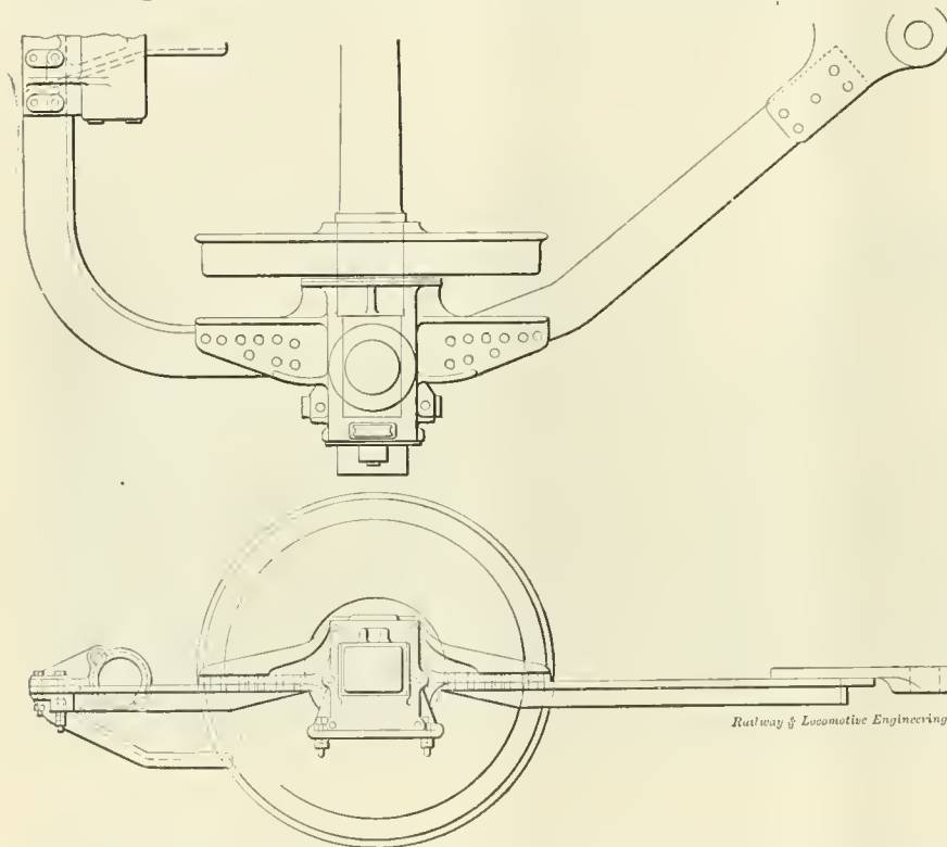
REAR OR CARRYING WHEEL TRUCK OF 4-6-2 ENGINE, N. Y. C. & H. R. R. R.
